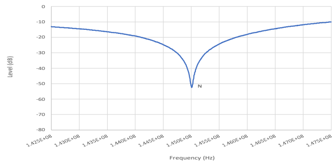
Return loss
